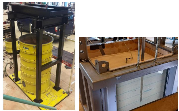
Figure 2: The Deltares calibration chamber (CC) test devices: (left) cylindrical CC and (right) half-CC with glass.
