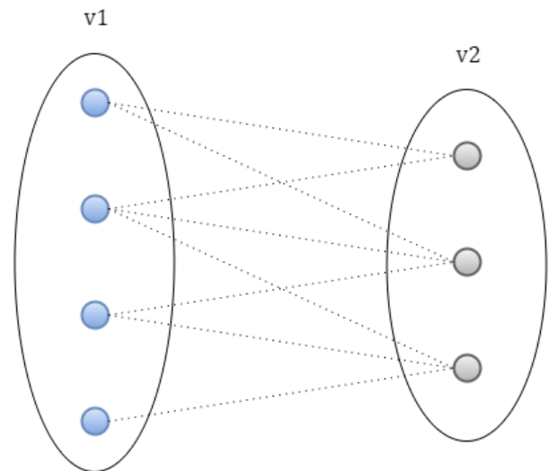
FIGURE 5. Example of a bipartite graph.
