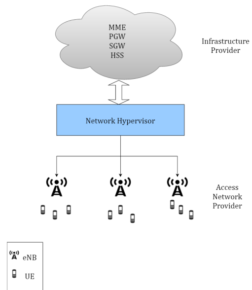
FIGURE 3. Core network virtualization.
