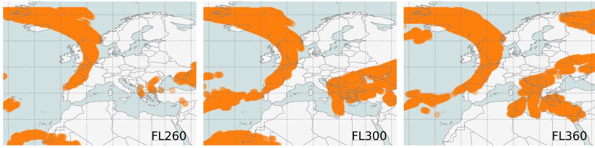
(a) ARPEGE forecast from the 6 th of January 2022 at 12:00 UTC, with a lookahead time of 3 hours.
