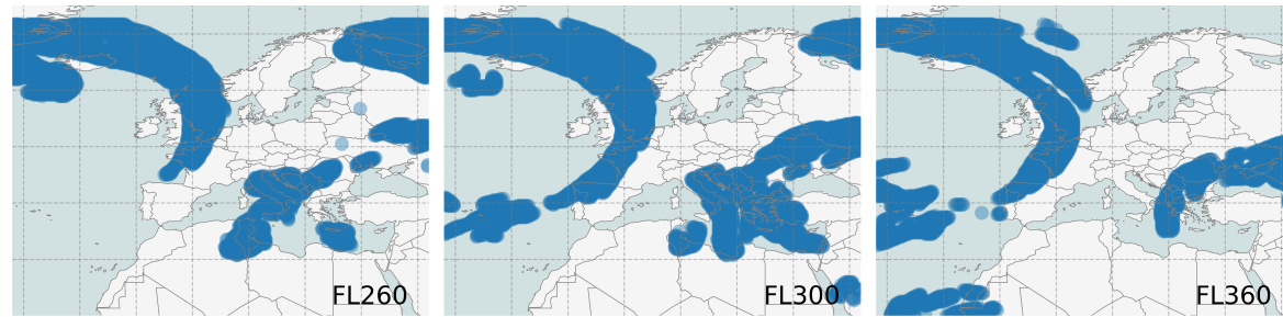
(c) ECMWF Reanalysis ERA-5 of the 6 th of January 2022, 15:00 UTC.
