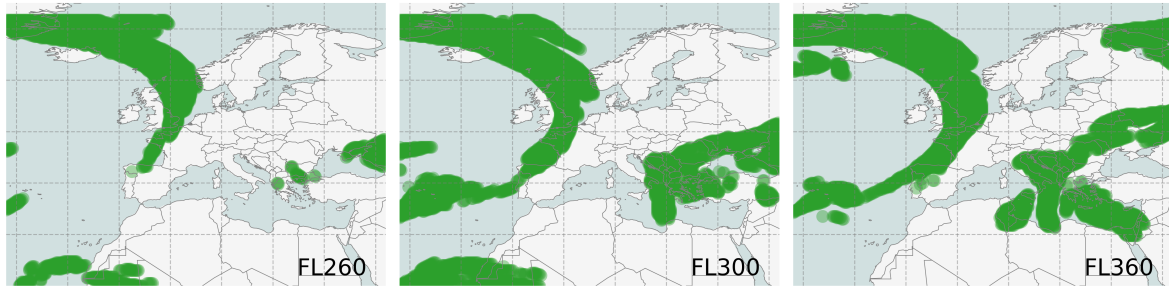
(b) ARPEGE forecast from the 6 th of January 2022 at 06:00 UTC, with a lookahead time of 9 hours.
