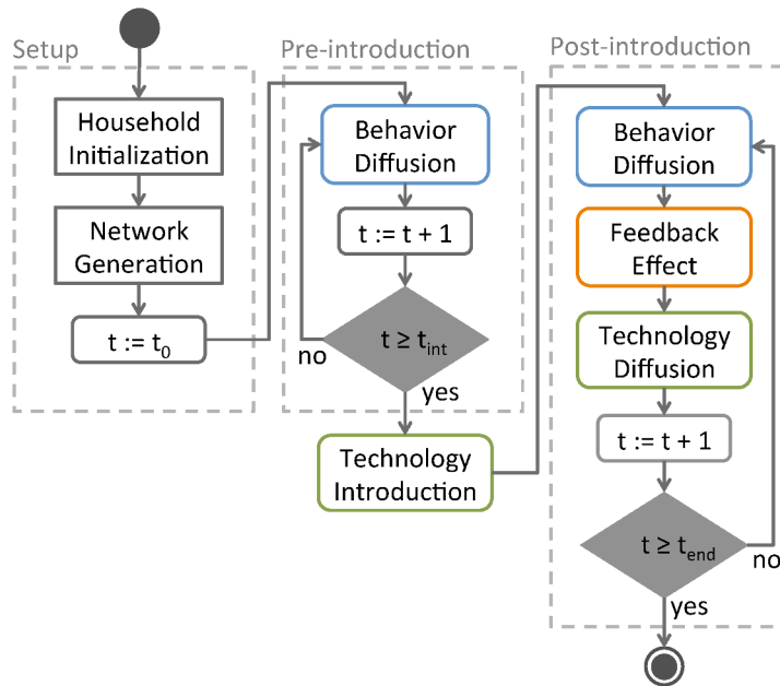
Figure 3.3: Simulation phases and scheduling. Formatted as a Unified Modeling Language activity diagram. See text for details.
