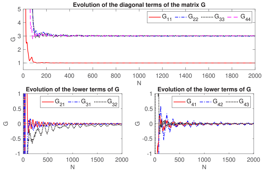
Fig. 6. Gaussian noise: evolution of the terms of the matrix G with the number of lines of the instrumental matrix W . An arbitrary value of the pixel size, \Delta y = 15 \mu m , was used for this simulation. The wavelength was set to 0.35 \mu m . To point out the trend of the G terms, the maximum value of N was fixed now to 2000.
