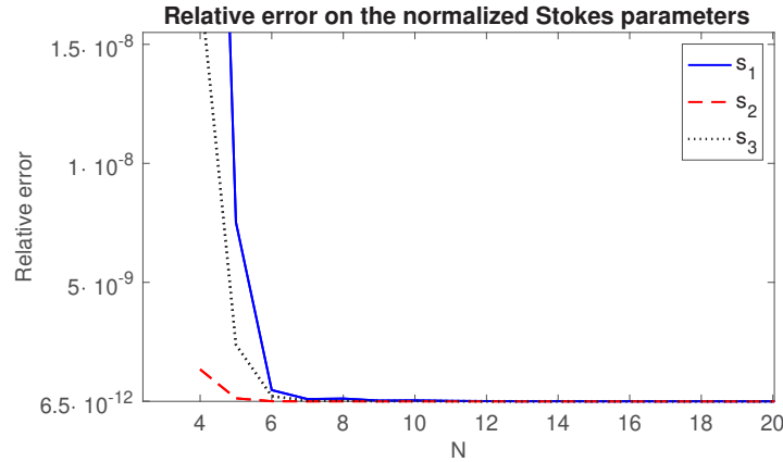
Fig. 3. Relative error on the normalized Stokes parameters as a function of the number of pixels, N . For these simulations, the size of the pixel was considered to be \Delta y = 10\mu\text{m} , the wavelength, \lambda = 0.35\mu\text{m} , whereas the incoming normalized polarization was arbitrarily chosen as \vec{s} = (1, 1/\sqrt{3}, 1/\sqrt{3}, 1/\sqrt{3})^T .
