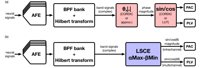
Fig. 1. System diagram of (a) a conventional PLV/PAC extraction unit and (b) the proposed PLV/PAC extraction unit with light sine and cosine extractor (LSCE) and \alpha\text{Max-}\beta\text{Min} magnitude approximation.
