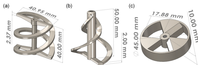
Fig. 13. Configurations of advanced stirrers (a) ribbon type stirrer (b) spiral type stirrer (c) rotary disc.
