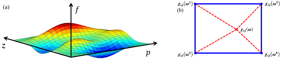
Fig. 7. Schematic description of operator parameterization and interpolation process for \chi operators with a predefined OBL resolution (modified from Voskov (2017); Lyu et al. (2021a)). \omega^1 to \omega^4 are four supporting points, and \omega is the current thermodynamic state of a given control volume at a given timestep in the simulation. (a) Operator distribution and (b) interpolation.
