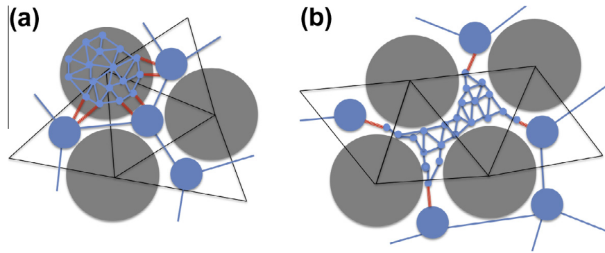
Fig. 5. Schematic of two-scale pore network construction for (a) grain-filling and (b) pore-filling microporosity (Mehmani and Prodanović, 2014).
