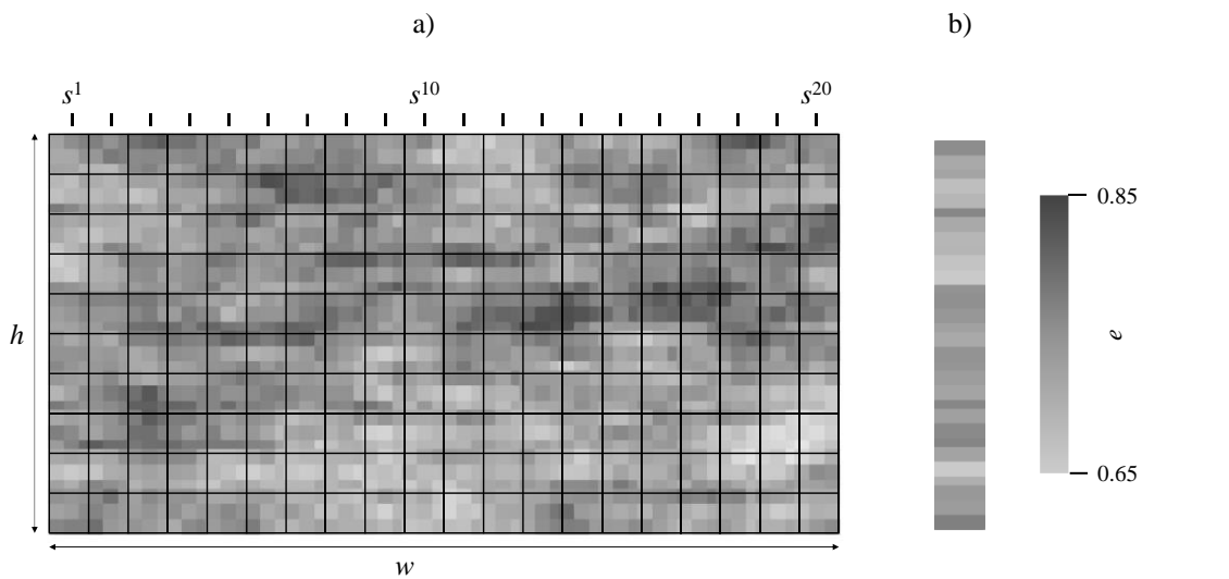
Figure 3. Typical void ratio e distribution over a) the 2D domain, and b) a 1D column.
