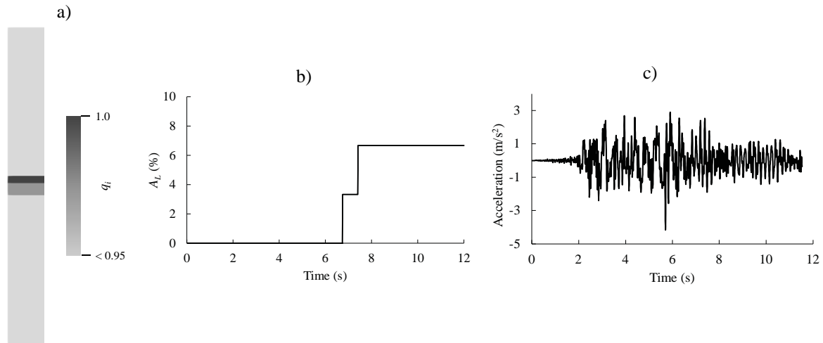
Figure 2. 1D column deterministic D solution: a) liquefaction index q_i after earthquake, b) liquefaction area A_L in time, and c) surface accelerations.
