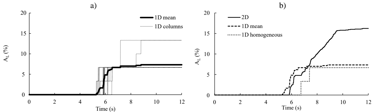
Figure 6. Liquefaction area ( A_L ) of the a) 1D columns and the computed 1D mean, and b) the 2D domain, the computed 1D mean and the homogeneous 1D column using e_\mu = 0.75 .
