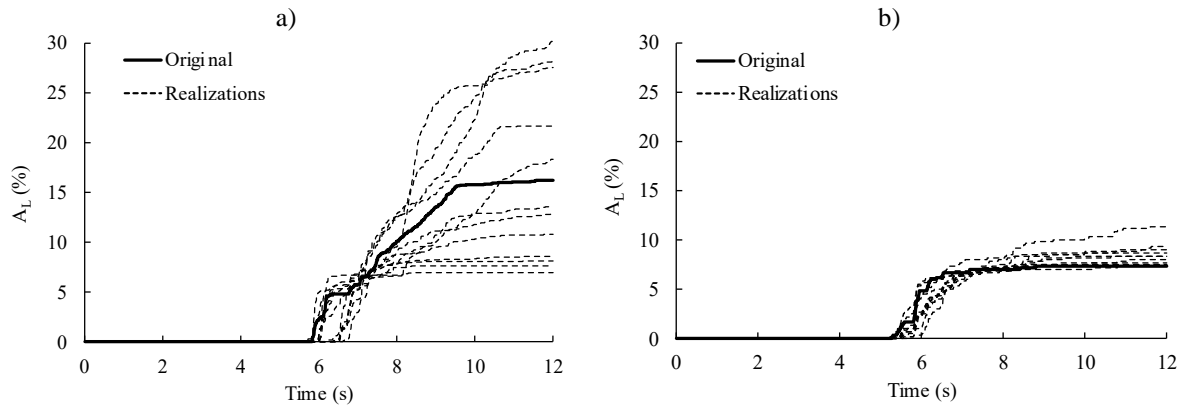
Figure 7. Liquefaction area ( A_L ) of a) 2D simulations, and b) their equivalent mean values using 1D columns.
