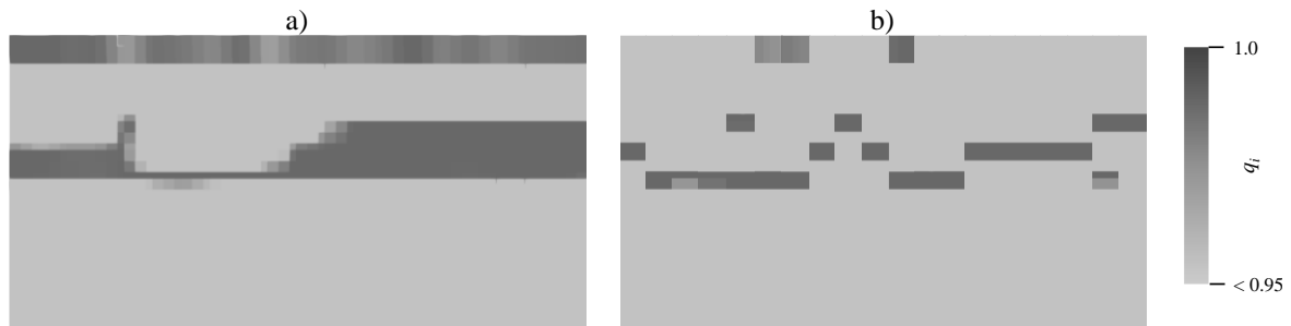
Figure 5. Final liquefaction stage of the a) 2D domain, and b) the combined 1D columns.
