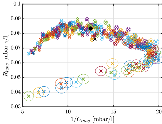
Fig. 10. Simulation results that contains the lung resistance and compliance estimates for 300 double breaths where the breathing effort amplitude variance is 0.14 [mbar 2 ] and \Delta IPAP is 1 [mbar]. The estimates together with their 95%-confidence intervals are shown. The true parameter values are displayed with (★) and the estimate average is displayed with the black cross (x). The difference between the true parameters values and the average estimated parameters indicate that a bias is present.
