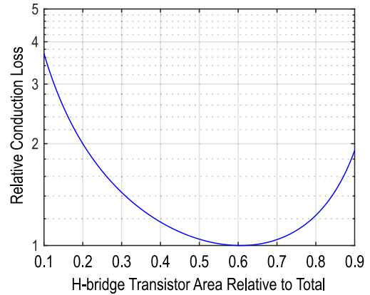
Fig. 9. Conduction loss as a function of the area allocated for H-bridge transistors M5 – M8 in the output stage.
