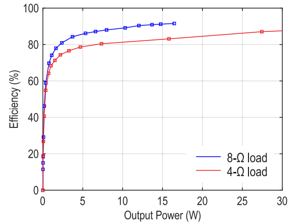
Fig. 19. Measured power efficiency at different output powers.
