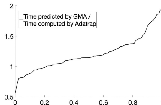
Fig. A1. Distribution of the ratio between times predicted by GMA and by ADATRAP.
