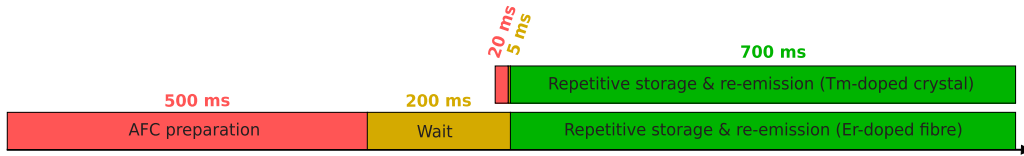
FIG. 5. Timing of experimental sequences in terms of synchronized preparation, wait and storage periods for the two memories.
