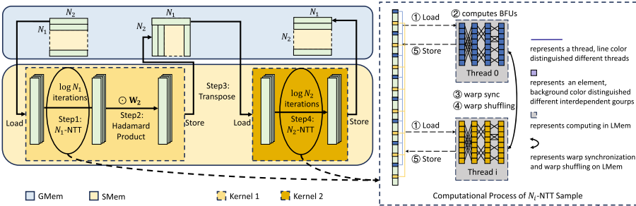
Fig. 4. The 4-step NTT dataflow. Note that: (1) The first three steps are fused into Kernel 1, and the last step occupies Kernel 2; (2) The zoom-in on the right can represent the N_1 and N_2 -NTT dataflow; (3) Each warp handles a full N_i -NTT sample, the elements in each N_i -NTT sample are split into different independent groups (eight elements in the same color are in the same group), and each thread processes one interdependent group; (4) Threads are synchronized on warp level, and the data are swapped using warp-shuffling.
