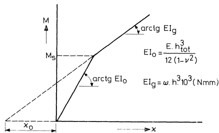
Fig. 12. Moment-curvature relationship for reinforced concrete.
