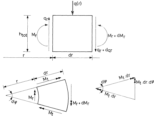
Fig. 51. Forces acting on a slab element.
