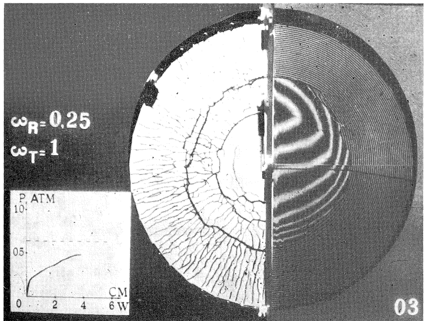
Fig. 8, Fig. 9. Collapse patterns of slabs 02 and 03; freely supported, loaded over entire area (uniformly distributed load).
