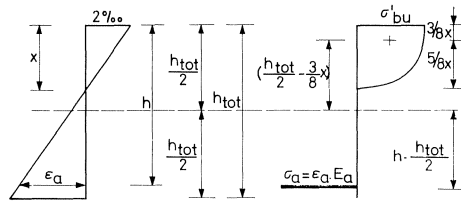
Fig. 46. Determination of M (in relation to middle plane) and the associated N' (normal force).
