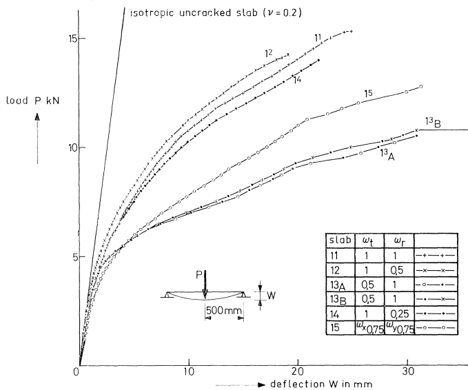
Fig. 10. Assembled test results of the circular slabs.
