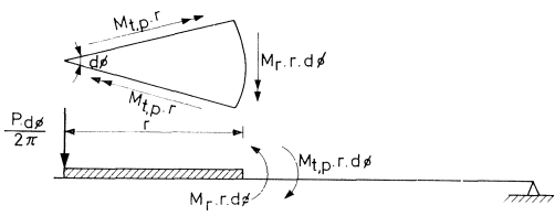
Fig. 25. Equilibrium of a slab segment where M_{t,p} has been reached in the tangential direction.
