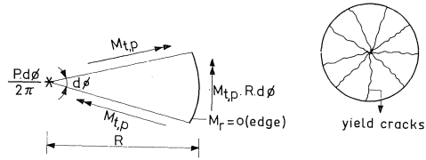
Fig. 22. Equilibrium of a slab segment at collapse, according to Johansen (point load).
