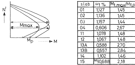
Fig. 44. Relationship between N' and M and the ratio between M_{t,max} and M_{t,p} .
