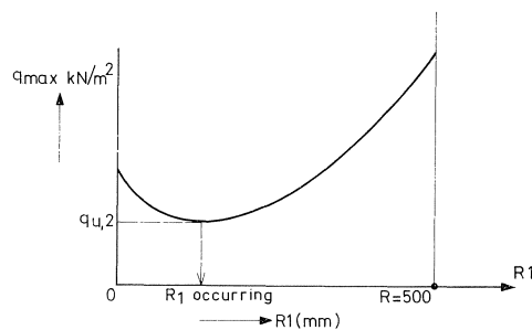
Fig. 43. Maximum load ( q_{max} ) as a function of the position of the tangential crack ( R_1 ) (slabs 01, 02 and 03).
