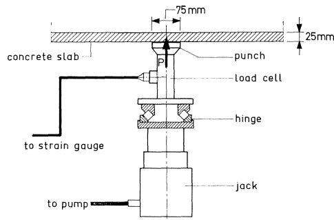
Fig. 6. Method of applying the point load.
