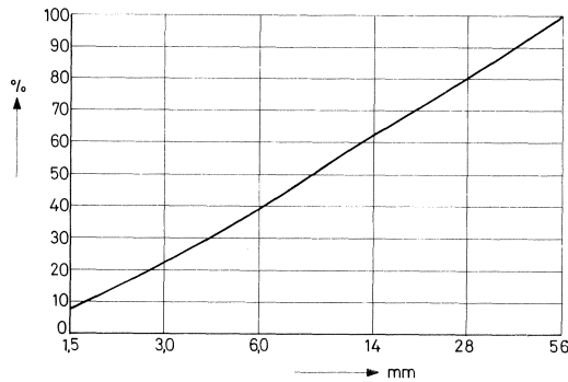
Fig. 47. Grading curve.
