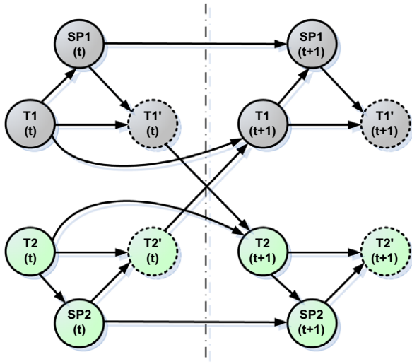
Fig. 1. Modeling of fire propagation in DBN in presence of sprinkler system.
