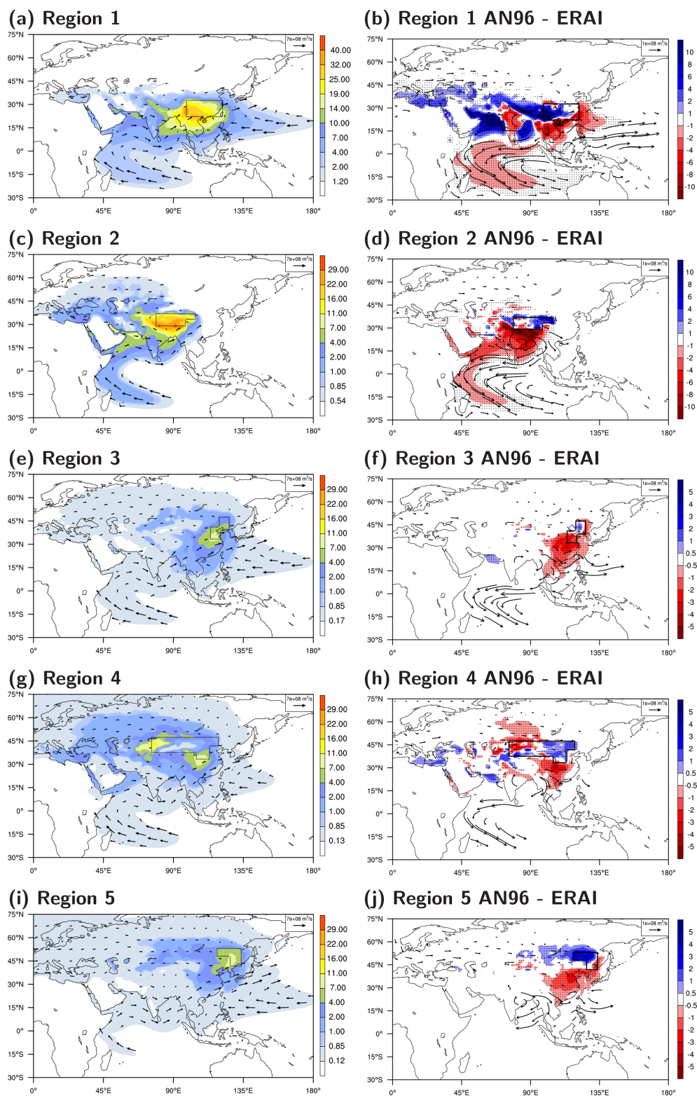
Figure 4. Annual mean moisture source for EA subregions (a, c, e, g and i; units: mm per month) and vertically integrated moisture flux (vector; units: \text{m}^3 \text{s}^{-1} ) calculated from ERA-Interim. Moisture source accounts for 80 % of precipitation are shown. Difference in annual mean moisture sources between AN96 and ERA-Interim (b, d, f, h and j; units: mm per month). The black box in each panel indicates the target region.
