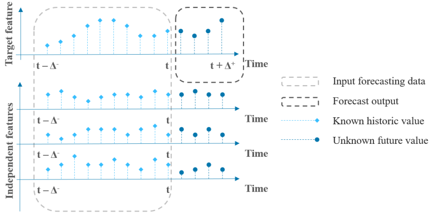
Figure 3: Data-Driven proposed framework for forecasting
