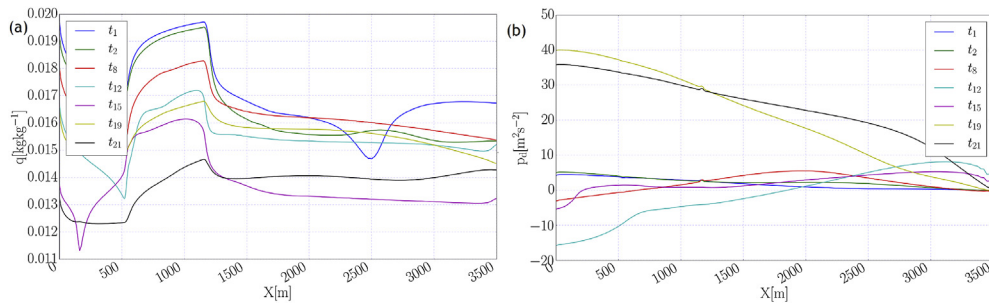
Fig. 14. Simulated flow parameters at height 2 m above the bottom surface in streamwise ( x -)direction include land and water surface. Water surface extends from x \approx 550 to x \approx 1200 m. Results are plotted for seven different times: t_1 = 01 : 00 , t_2 = 02 : 00 , t_8 = 08 : 00 , t_{12} = 12 : 00 , t_{15} = 15 : 00 , t_{19} = 19 : 00 and t_{21} = 24 : 00 hr; (a) specific humidity; and (b) dynamic pressure ( P_d = P_{total} - P_{static} ).
