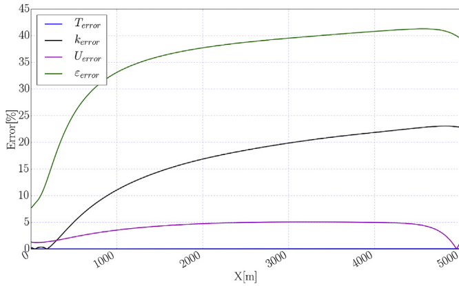
Fig. 8. Relative change of flow parameters in stable atmospheric condition relative to inlet values.
