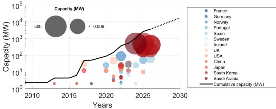
Fig. 1 Existing and planned floating wind projects worldwide: bubbles are projects in the pipeline as of 2021 (data from DOE (2021)), the continuous line shows the cumulative capacity (in MW) of these projects, and the dashed line is the ambitions to reach in Europe alone by 2030 (data from WindEurope)
