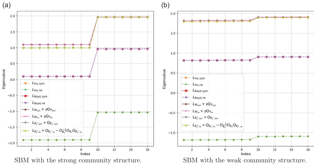
Figure 5. SBM with strong and weak community structure: spectra of L_{Hu, sym} , L_{Hu, rw} , L_{Boyd, sym} , L_{Boyd, rw} and four choices of L_{mix} \in \{L_{W_{sym}} + \gamma Q_{P_{sym}}, L_{W_{rw}} + \gamma Q_{P_{rw}}, L_{B_{1, sym}}^+ + Q_{B_{1, sym}}^-, L_{B_{1, rw}}^+ + Q_{B_{1, rw}}^- - D_{B_1}^{-1} D_{B_1} Q_{B_{1, rw}}^-\} with \gamma = 1 and the NG null model, for a single realisation of an SBM with 10 blocks. The following graphs overlap: L_{Hu, sym} and L_{Hu, rw} ; L_{Boyd, sym} and L_{Boyd, rw} ; L_{W_{sym}} + \gamma Q_{P_{sym}} and L_{W_{rw}} + \gamma Q_{P_{rw}} (which is expected thanks to Remark 5.2); L_{B_{1, sym}}^+ + Q_{B_{1, sym}}^- and L_{B_{1, rw}}^+ + Q_{B_{1, rw}}^- - D_{B_1}^{-1} D_{B_1} Q_{B_{1, rw}}^- (which is expected from Remark 5.3).
