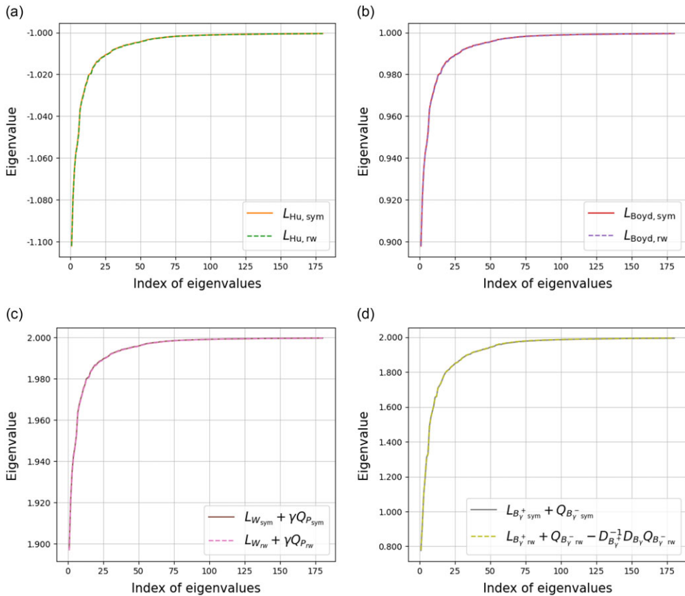
Figure 1. MNIST: comparison of the spectra of different operators with \gamma = 1 under the NG null model. In each of the plots, one of the two curves is hidden behind the other one.
