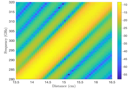
(b) Received power (dB) with \phi_{\text{std}}(x, y) .
