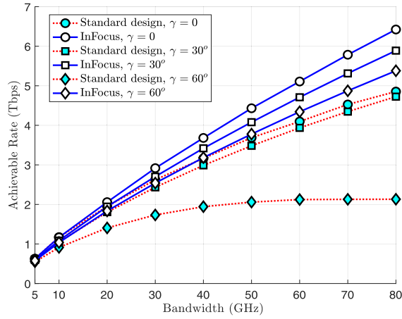
(a) Rate with the operating bandwidth B .
