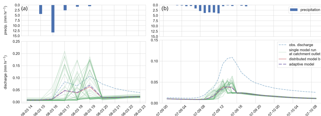
Figure 7. (a) Rainfall-runoff event I and (b) rainfall-runoff event II. Blue bars in the upper panel show the average precipitation of the precipitation field for each time step ( \text{mm h}^{-1} ). The green curves in the lower panel represent a single gridded model of the distributed model b, the red line the area-weighted mean of the distributed model, the dashed purple line the area-weighted mean of the adaptive model, and the dashed blue line the observed specific discharge of the Colpach.
