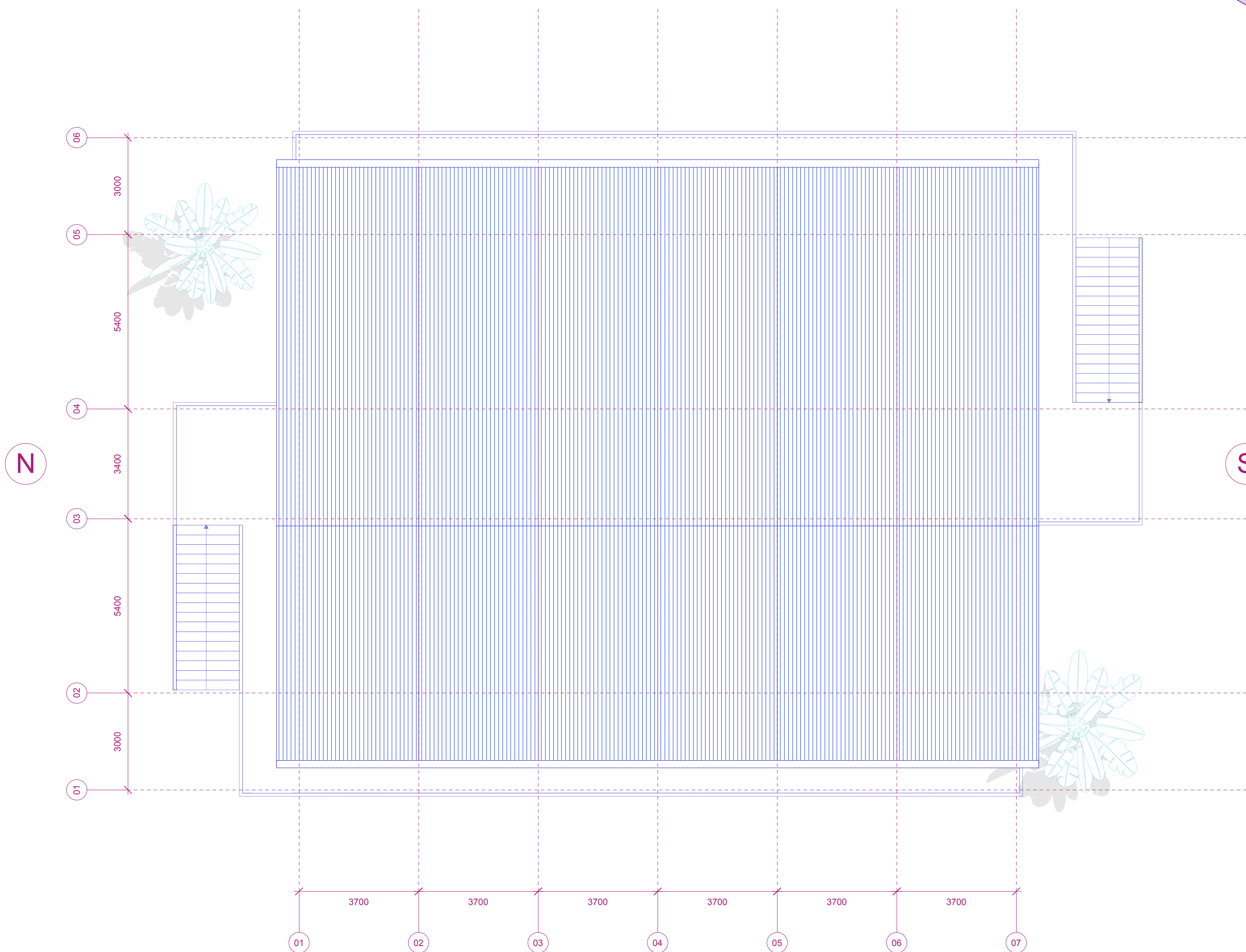
ROOFPLAN +7
