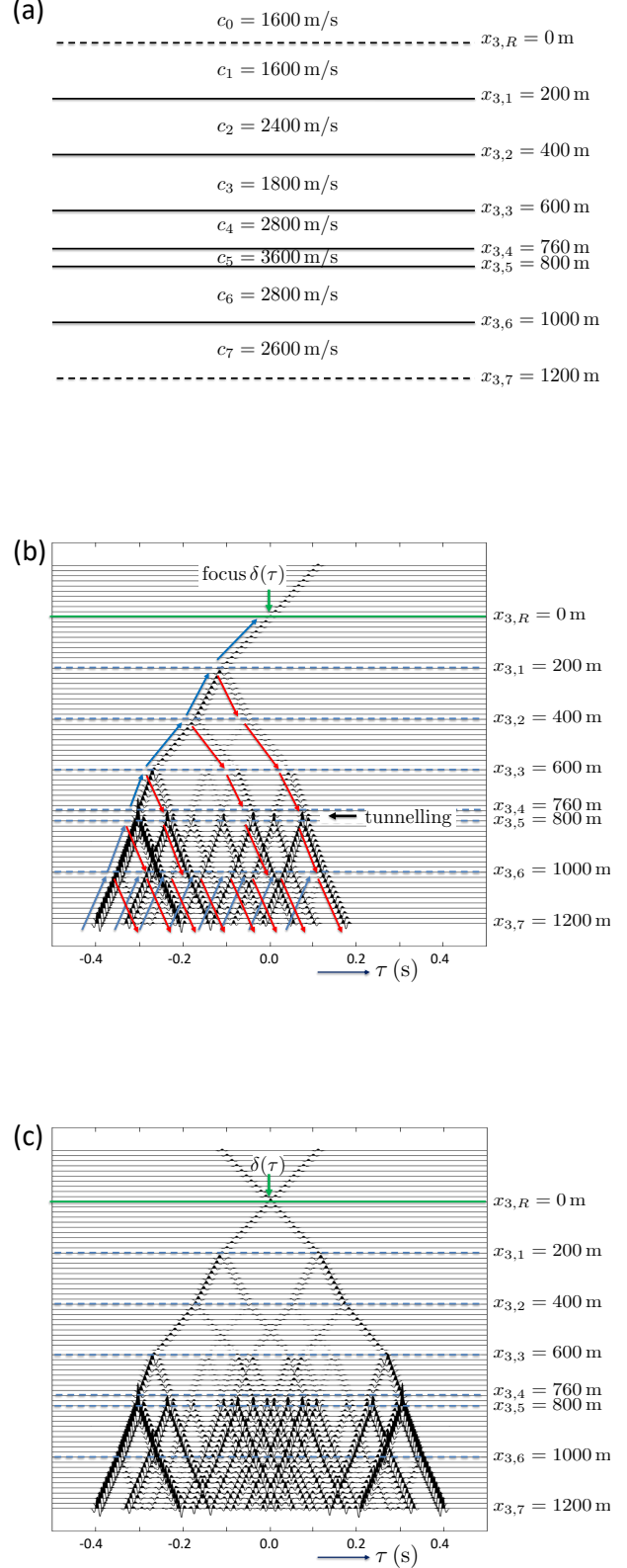
Figure 2: (a) Horizontally layered medium. (b) Focusing function F^p(s_1, x_3, x_{3,R}, \tau) (for fixed s_1 ). (c) Propagator matrix element W^{p,p}(s_1, x_3, x_{3,R}, \tau) (for fixed s_1 ).
