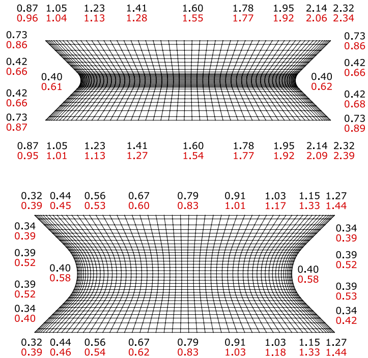
Fig. 12. Measurements on the local thickness of the two prototypes (red) is compared to the local thickness of the optimized modeled geometry (black). Measurements are only performed on the accessible perimeter of the shells.
