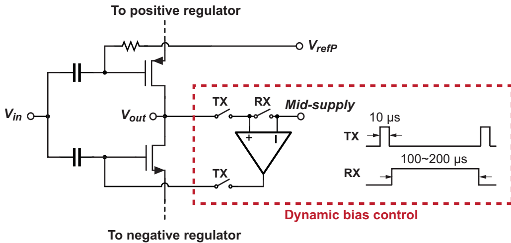
Fig. 7 Dynamic bias control scheme.
