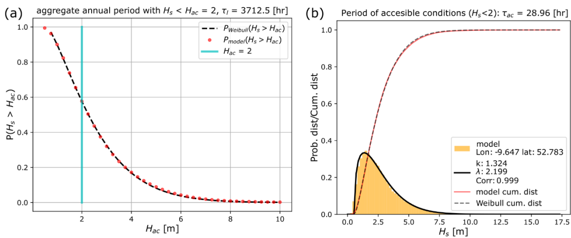
Figure 17: (a) Wave height Probability of exceedance from Weibull best fit and from modelled time series. (b) wave height density probability distribution from modelled time series and Weibull fit.
