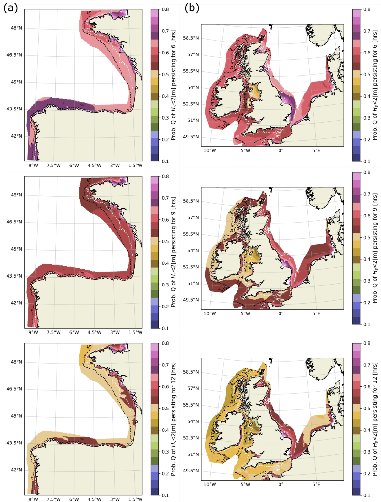
Figure 21: Estimated yearly prob. of occurrence Q of H_s < H_{ac}=2 m for continuous time windows of 6, 9 and 12 hrs (top, mid and bottom panels respectively). (a) Portugal and Bay of Biscay, (b) Ireland, UK and North Sea.
