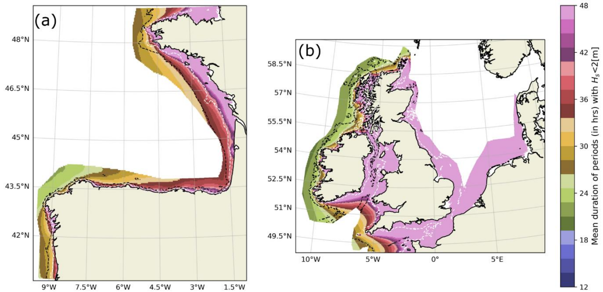
Figure 20: Estimated yearly \tau_{ac} , mean duration of periods with H_s < H_{ac}=2 m.
