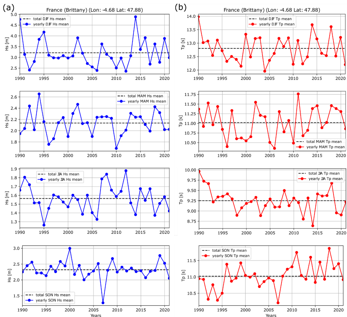
Figure 70: (a) H_s and (b) T_p yearly mean seasonal values compared to the 32-years mean. Location: Brittany (France).
