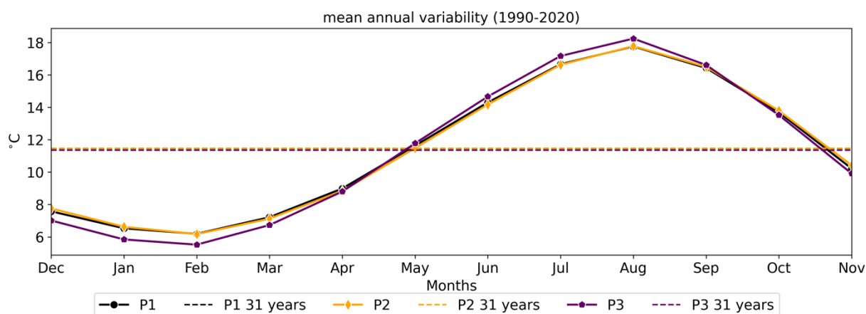
Figure 53: Same as Figure 54, but for the Ireland region.
