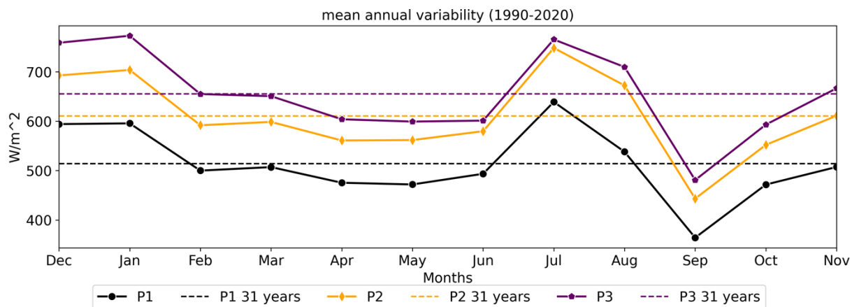
Figure 42: Time-series of 100 m wind power density computed during each month, at points P1, P2, and P3, over the Iberia region. Horizontal dashed lines represent the overall statistics at the respective points.
