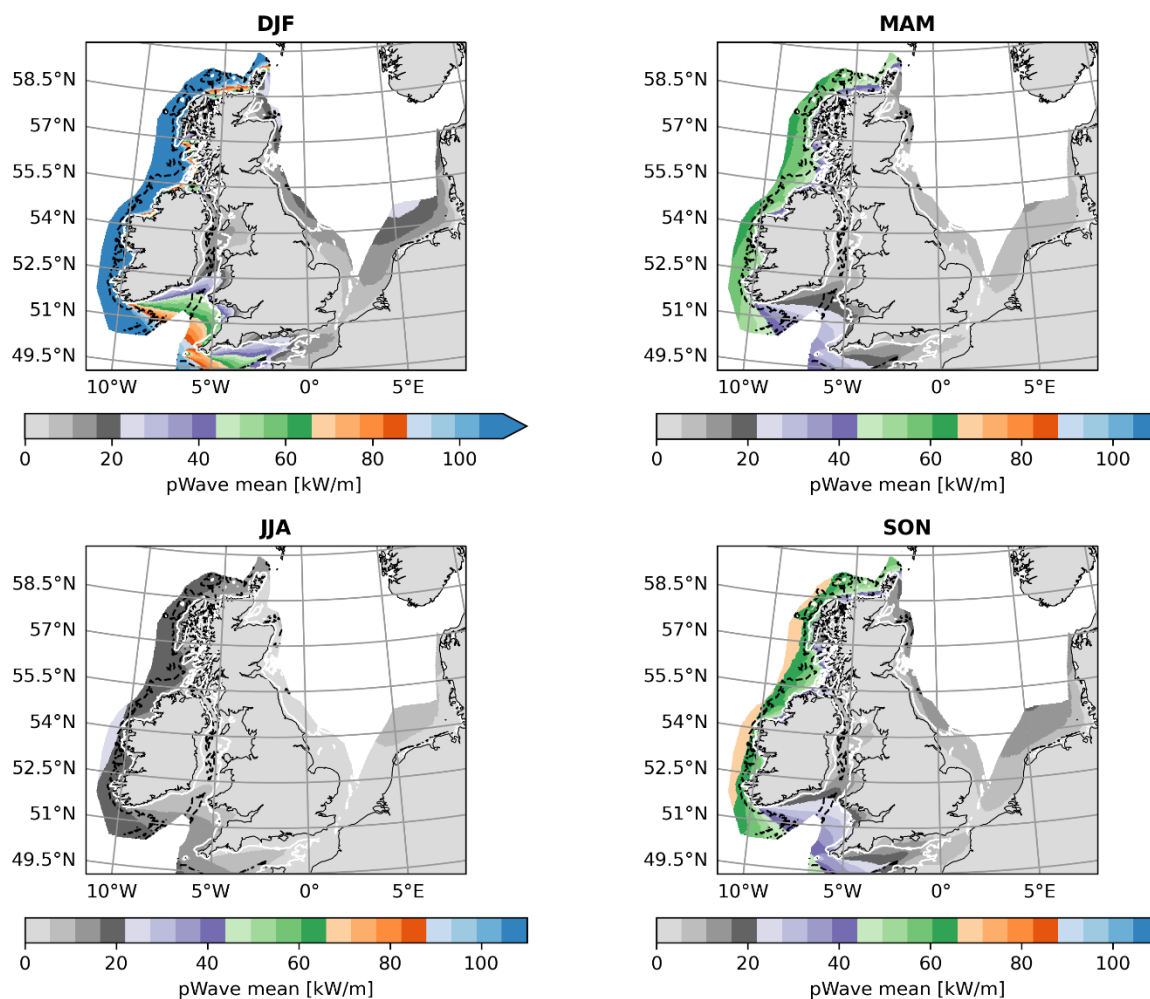
Figure 25: H_s 32-years pWave seasonal mean for Ireland, UK and The North Sea.
