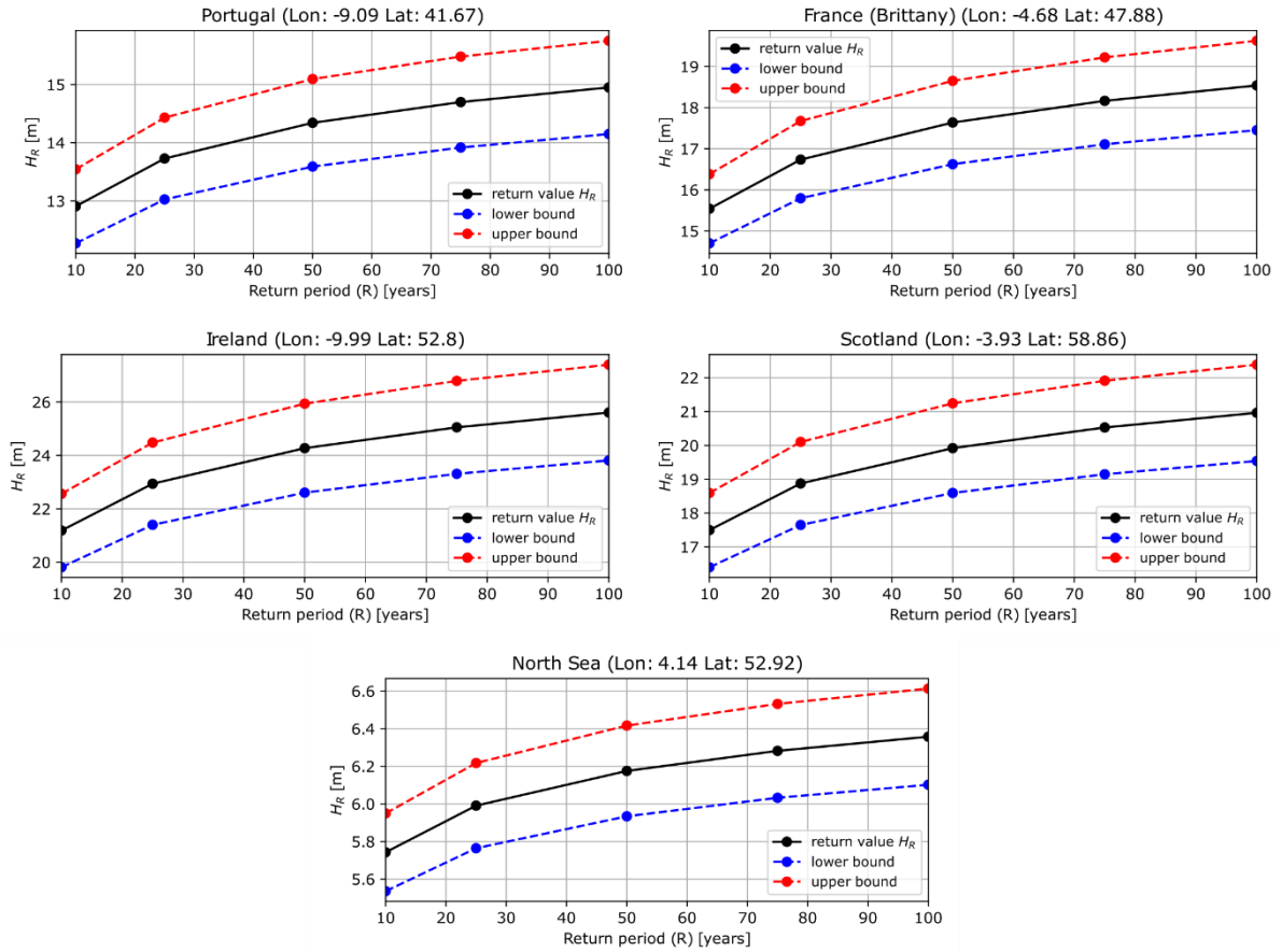
Figure 16: Return value H_R and 90% confidence interval bounds.
