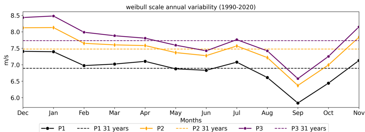
Figure 66: Time-series of 10 m wind Weibull scale parameter computed during each month, at points P1, P2, and P3, over the Iberia region. Horizontal dashed lines represent the overall statistics at the respective points.
