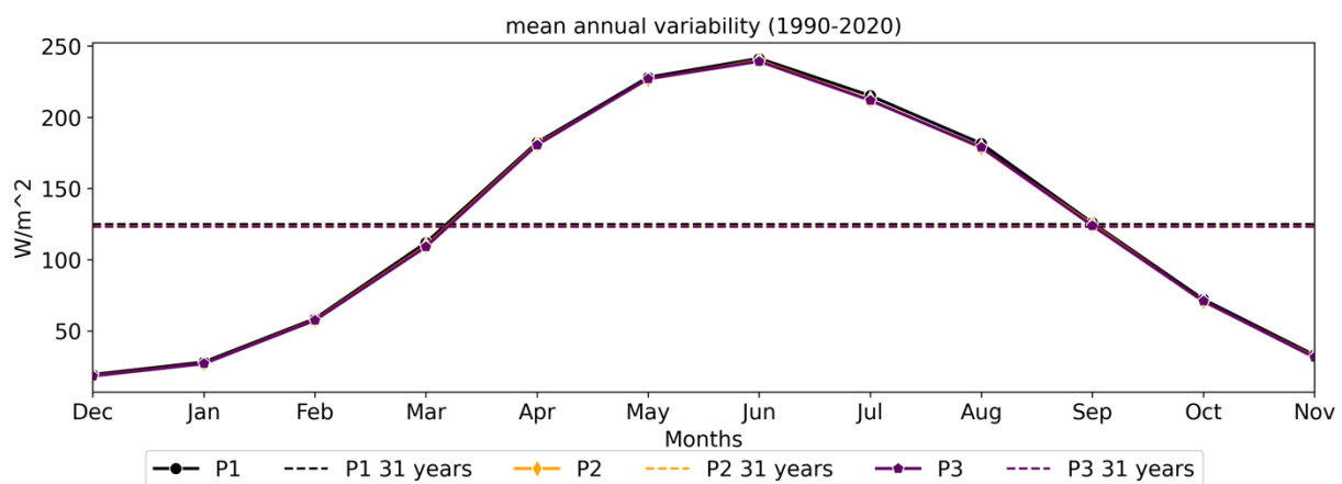
Figure 61: Same as Figure 60, but for the Ireland region.
