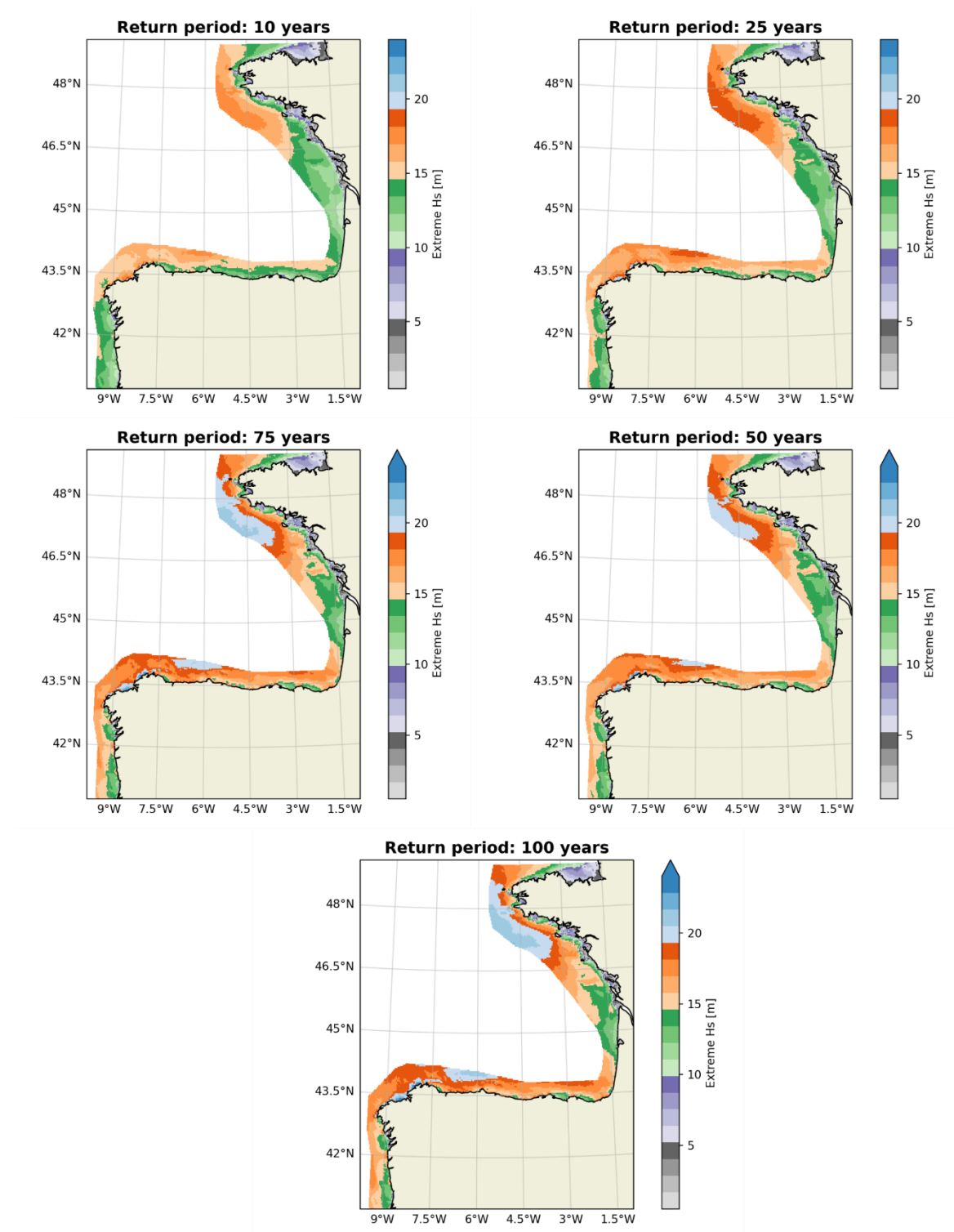
Figure 12: Expected extreme significant wave height return value ( H_R ) for 10, 25, 50, 75, and 100 years return periods. Portugal and Bay of Biscay.
