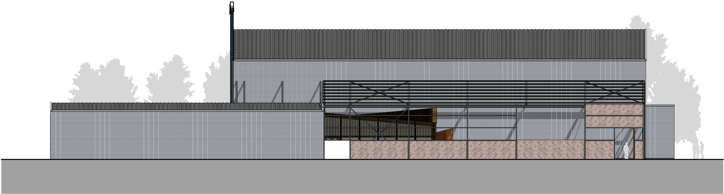
East Elevation
