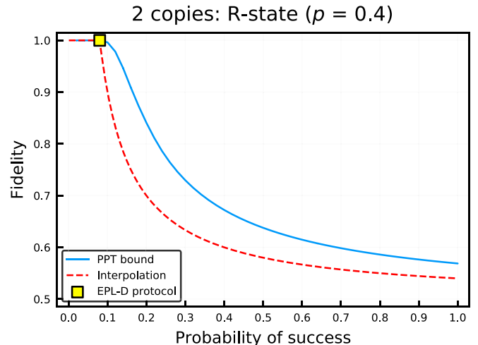
FIG. 9. Distilling the R states \tau_{ab}^{\otimes 2} with D = 2 and p = 0.4 in Eq. (42) to a two-qubit state. The fidelity of the input copy is F_{in} = 0.4 and we observe that deterministic distillation (with p_{succ} = 1 ) which achieves output fidelity larger than half is easily achievable for two copies of this state. We also see that EPL-D allows for achieving unit fidelity even if p \leq 0.5 . The 1-BSE bound is not included because it overlaps with the PPT bound.
