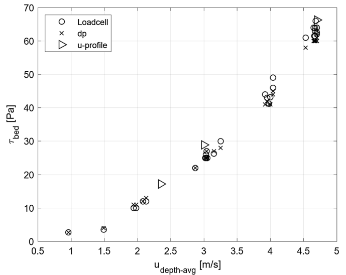
Fig. 9. Determined bed shear stresses as a function of the flow velocity.
