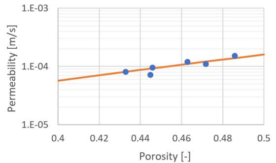
Fig. 4. Permeability ( k ) as a function of the porosity n_0 .
