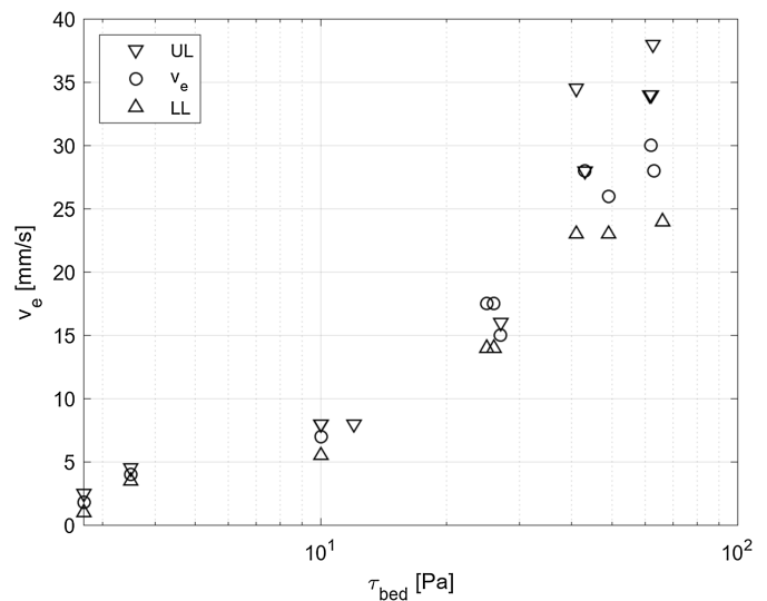
Fig. 10. Determined erosion velocity (and corresponding upper and lower limits) as a function of the measured bed shear stress.
