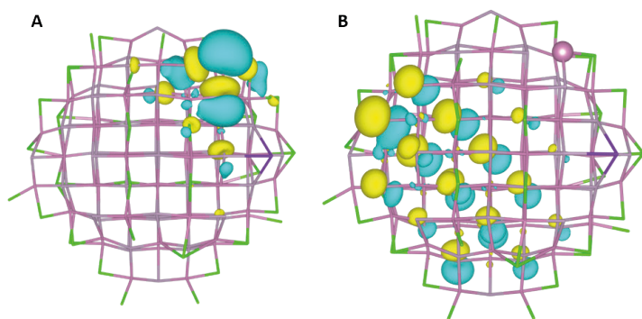
Figure A3.3. A) Contour plot of the LUMO of the \beta MOs of the spherical core-only InP QD for n = 1 using a contour plot value of 0.005 \text{ e/bohr}^3 . B) Contour plot of the HOMO of the \beta MOs of the spherical core-only InP QD.
