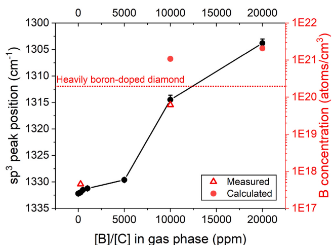
Fig. 5. The variation of the \text{sp}^3 -carbon Raman peak (black) and the boron concentration in the BDD sheets (red) as a function of the boron level in the gas phase. The calculated B-concentration data in the samples were derived from Raman spectral data whereas the measured data were derived from SIMS and Hall-effect measurements. The error bars represent the standard error of the mean. The standard error of the mean boron concentration did not exceed 4 % of the mean value.
