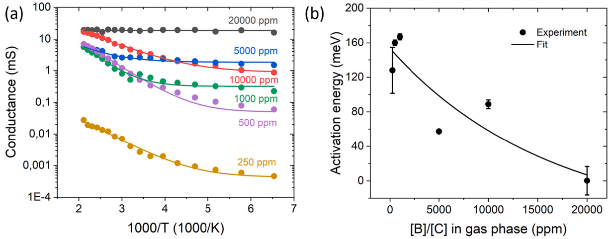
Fig. 6. Electrical measurements as a function of temperature and [B]/[C] ratio in the gas phase: (a) conductance of the diamond sheets versus 1000/T, (b) extracted activation energies calculated for the high-temperature range ( > 393 K) with exponential fitting curve. The standard error of the mean conductance did not exceed 2.5 % of the mean value for a single measurement.
