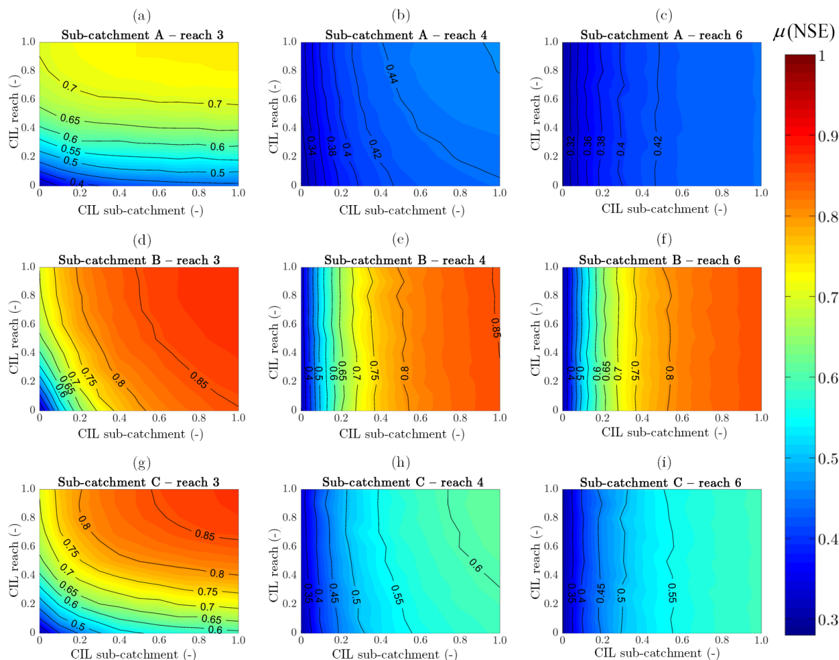
Figure 5. The \mu(\text{NSE}) values obtained by assimilating CS observations from a combination of StSc sensors located in different sub-catchments and river reaches with 4 h lead time in the case of different CIL values.
