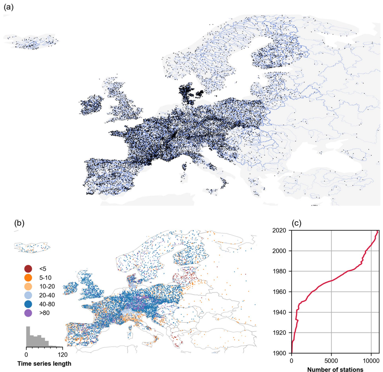
Fig. 2 (a) Spatial distribution of the 17,130 streamflow gauges currently included in EStreams (in black dots) with their catchment boundaries in background (in blue) over Europe. (b) Spatial distribution of the streamflow with the colors representing the time series length in years. (c) Temporal evolution of station coverage. The plot shows the number of active stations in a given year. Although the curve accounts for dismissed stations, it still shows an increasing trend. Basemap from GeoPandas 104 .
