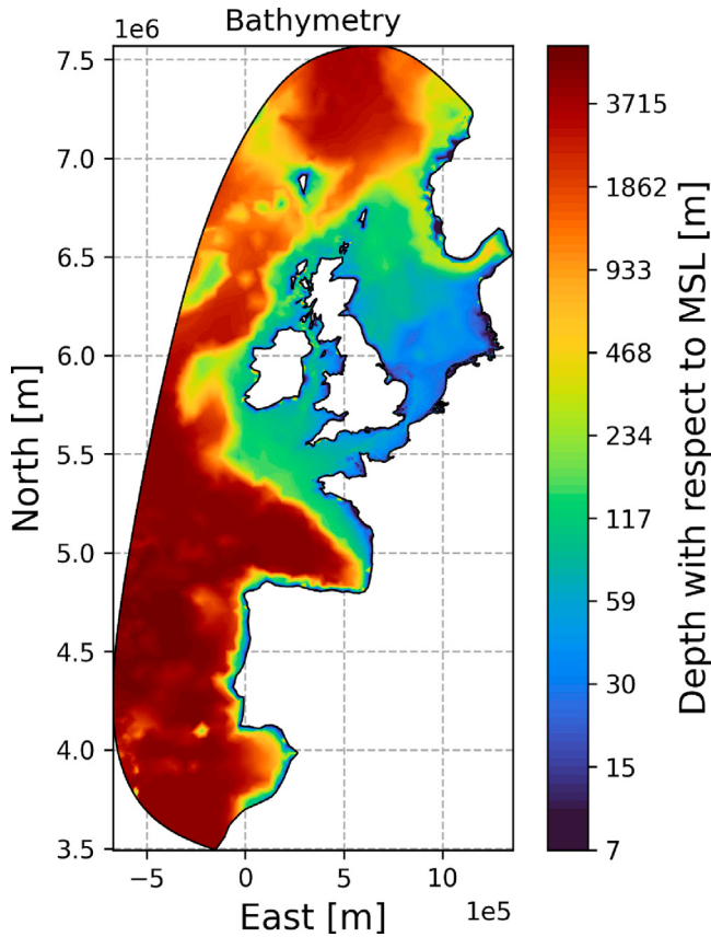
Fig. 2. Bathymetry of the domain in meters with regards to mean sea level as provided by EMODnet [32].
