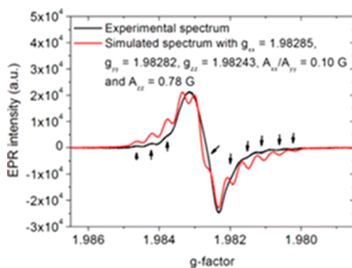
Figure 15. Left shows experimental (black) and simulated (red) EPR spectra of the end-on superoxido intermediate (with oxygen-17). Right shows the SOMO of the same species (oxygen-16). Reprinted from ref 420. Copyright 2016 American Chemical Society.
