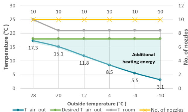
Figure 4. Graph showing the no. of nozzles and air temperature achieved at different outside temperatures.
