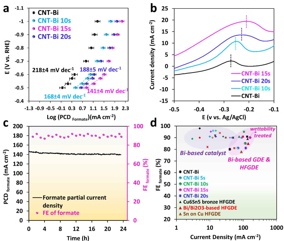
Fig. 4. a) Tafel plots of formate for dual-layer HFGDEs; b) Single oxidative LSV scans at 50 mV/s in N_2 -saturated 0.1 M; c) 24 h stability test at -1.0 V vs. RHE: faradaic efficiency and formate partial current density in the flow reactor with CNT-Bi 15 s dual-layer HFGDE; d) CO_2RR performance comparison of dual-layer HFGDEs with other Bi-based catalysts and GDEs/HFGDEs for formate production in neutral (bicarbonate) electrolytes with the same concentration (more details on CO_2RR performance and electrolyte type in Table S2).
