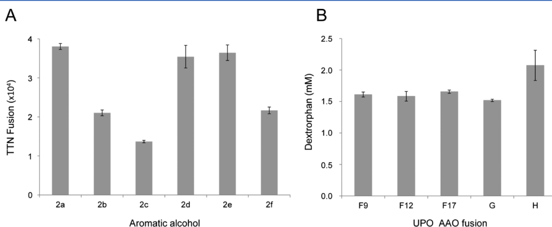
Figure 4. Aromatic alcohol selection and fusion enzyme performance in the production of dextromethorphan. (A) TTNs for the transformation of dextromethorphan into dextromethorphan. Reactions were performed in 1.5 mL GC vials in a final volume of 0.3 mL containing 10 mM of each aromatic alcohol, 0.04 \mu\text{M} of the H fusion (peroxygenase partner concentration measured with the CO difference spectrum), and 10 mM dextromethorphan hydrobromide in 100 mM potassium phosphate buffer at pH 7.0. (B) Comparison of the different UPO_AAO fusions with 2a and dextromethorphan. The reactions were performed in 1.5 mL GC vials in a final volume of 0.3 mL containing 10 mM 2a, 0.05 \mu\text{M} of each UPO_AAO fusion (a peroxygenase partner concentration measured with the CO difference spectrum), and 10 mM dextromethorphan hydrobromide in 100 mM potassium phosphate buffer at pH 7.0. All reactions were incubated for 24 h at 30 °C and at 600 rpm. The reactions were performed in duplicate at least and analyzed by GC-FID, as described in the Materials and Methods section.
