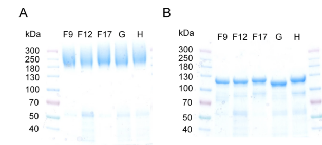
Figure 3. Molecular mass of UPO_AAO fusions. (A) Purified fusions and (B) fusions after treatment with PNGaseF resolved on 4–20% precast polyacrylamide gels.
