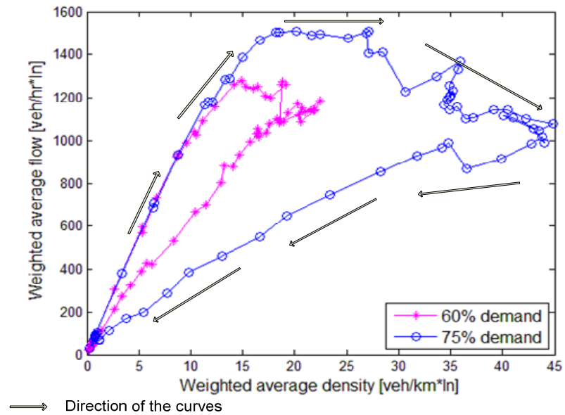
Figure 4.5: MFD of motorways at 60 and 75% demand level
