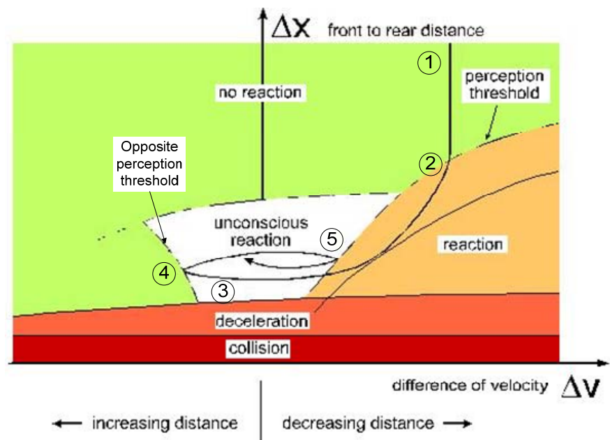
Figure A.2: Car following logic (PTV AG, 2007)
