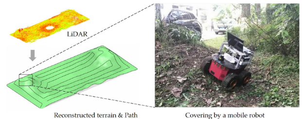
Fig. 10. Experiments taken in an outdoor environment for verifying the energy consumption by following a zig-zag path vs. a spiral path generated by our method (see the path shown on the reconstructed surface).
