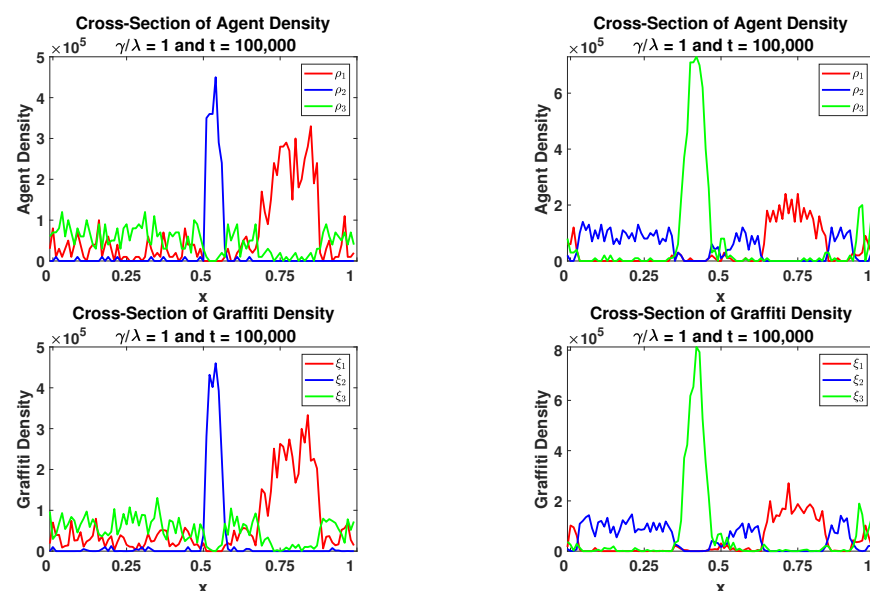
Figure 13. Cross-sectional slices of the agent and graffiti densities for different \beta_j extensions at the final time step for a segregated state. Here, we have N_1 = N_2 = N = 3 = 50,000 with \delta t = 1 and the lattice size is 100 \times 100 ; in both simulations, \beta_1 = 2 \times 10^{-5} , \beta_2 = 3.5 \times 10^{-5} and \beta_3 = 0.5 \times 10^{-5} . (Left): Here, we consider the Timidity variation of the model. We observe that the territories range from small and very dense, with little incursion from the other gangs, to large and spread out, with other gang members encroaching on the territory, as the gangs' \beta_j value varies from high to low. (Right): Here, we consider the Threat Level variation of the model. We see that the size of the territory here is correlated with the \beta_j value for the gang, and that all of the territories here seem well-defined, with little of the territorial encroachment seen in the model pictured on the left.
