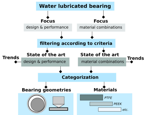
Fig. 5. Approach used to differentiate between geometry and material focused literature.
