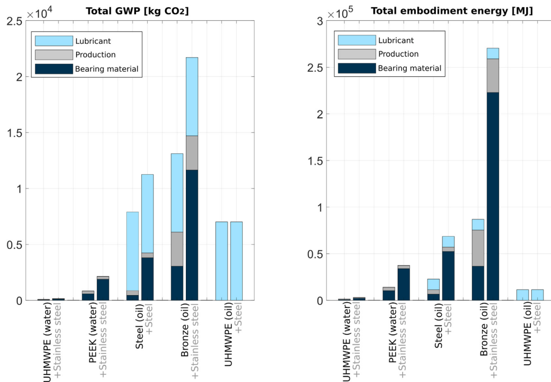
Fig. 13. Total GWP and embodiment energy for the 5 material/lubricant combinations analyzed in the case study. In all cases, both the worst and best case material scenario's (recycled or virgin) have been presented. Lubricated UHMWPE-stainless steel is 191.44 and 360.72 kg CO 2 , and the total embodiment energy equals 3335.72 and 6920.33 MJ respectively.
