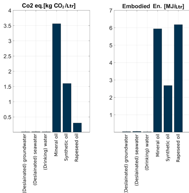
Fig. 12. CO 2 equivalent and Embodiment energy of several lubricants. Note that for deslaminated groundwater at 0.0016 [kg/CO 2 /ltr] & 0.027 [MJ/ltr], deslaminated seawater at 0.0025 water [kg/CO 2 /ltr] & 0.042 [MJ/ltr] and recycled drinking water at 0.0011 [kg/CO 2 /ltr] & 0.018[MJ/ltr] is significantly lower than any oil alternative.
