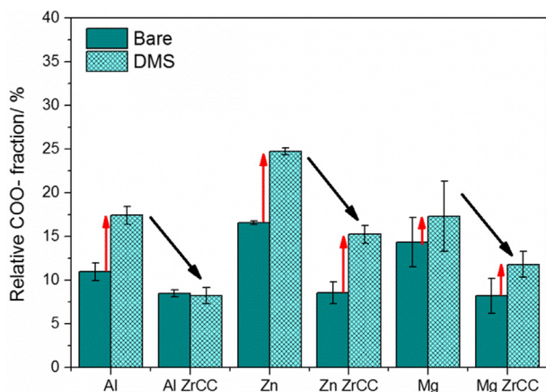
Fig. 16. Relative COO - fractions (%) at metal oxide surface before (bare) and after (DMS) dimethylsuccinate adsorption.
