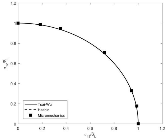
Figure 5. Stress envelope for combined longitudinal shear in two different planes.
