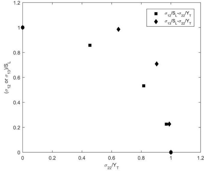
Figure 7. Stress envelopes for different combinations of longitudinal shear stresses with transverse normal stress.
