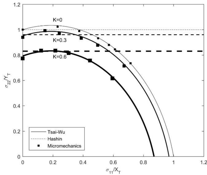
Figure 12. \sigma_{22} - \sigma_{11} Failure envelope accompanied with transverse shear stress ( K = \sigma_{23} / S_T ).
