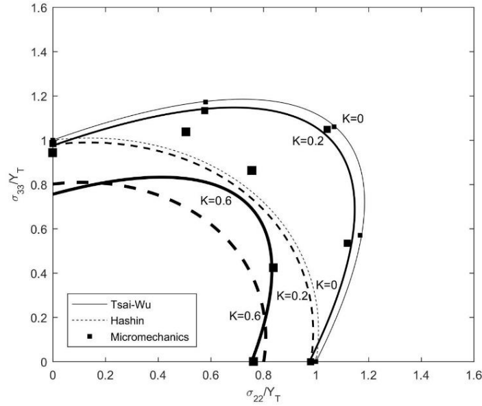
Figure 8. Failure surface of the composite subjected to biaxial transverse tension and longitudinal shear ( K = \sigma_{12} / S_L ).
