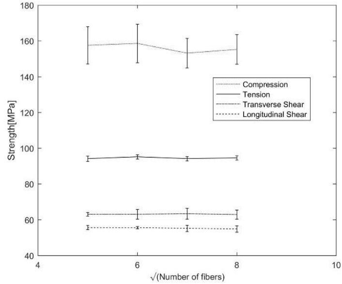
Figure 2. Mean and standard deviation of tensile, compressive, longitudinal shear and transverse shear strengths for 5 realizations for various RVE sizes.
