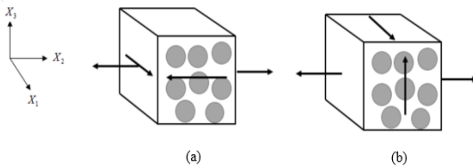
Figure 6. Combination of transverse normal stress with longitudinal shear stress applied (a) in the same plane, (b) in two different planes.
