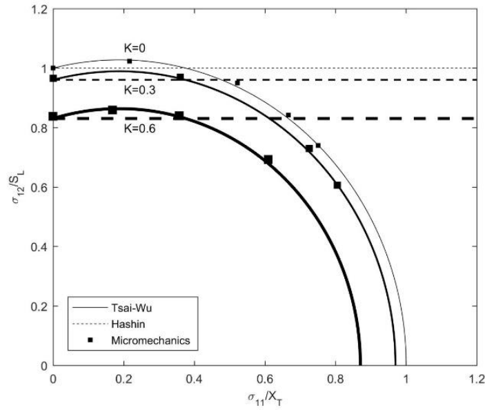
Figure 10. Stress envelope for combined longitudinal shear and fiber tension loadings for various K = \sigma_{23}/S_T ratios.
