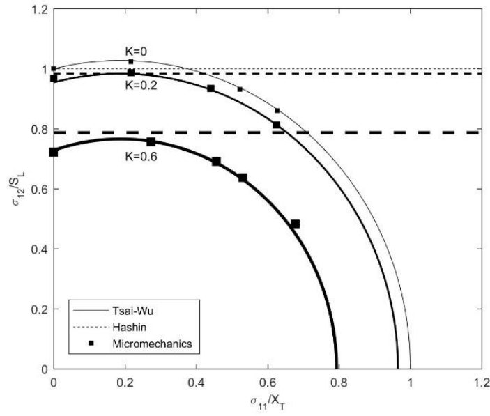
Figure 11. Longitudinal shear strength as a function of \sigma_{11} for different values of normal stress ratios ( K = \sigma_{22} / Y_T ).
