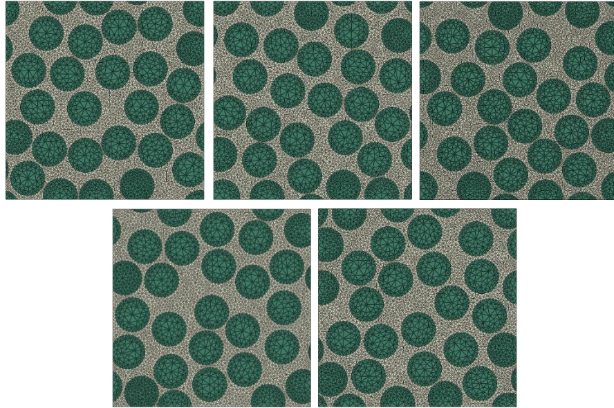
Figure 1. Five realizations of a fiber distribution with 25 fibers and their finite element discretization.
