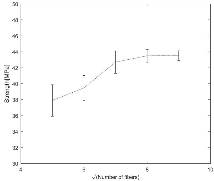
Figure 3. Mean and standard deviation of maximum longitudinal shear stress for 5 realizations for various RVE sizes in combined loading including longitudinal tension and longitudinal shear in two different planes.
