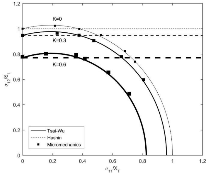
Figure 9. Variation of longitudinal shear strength with respect to the longitudinal axial tension for various K = \sigma_{13} / S_L ratios.
