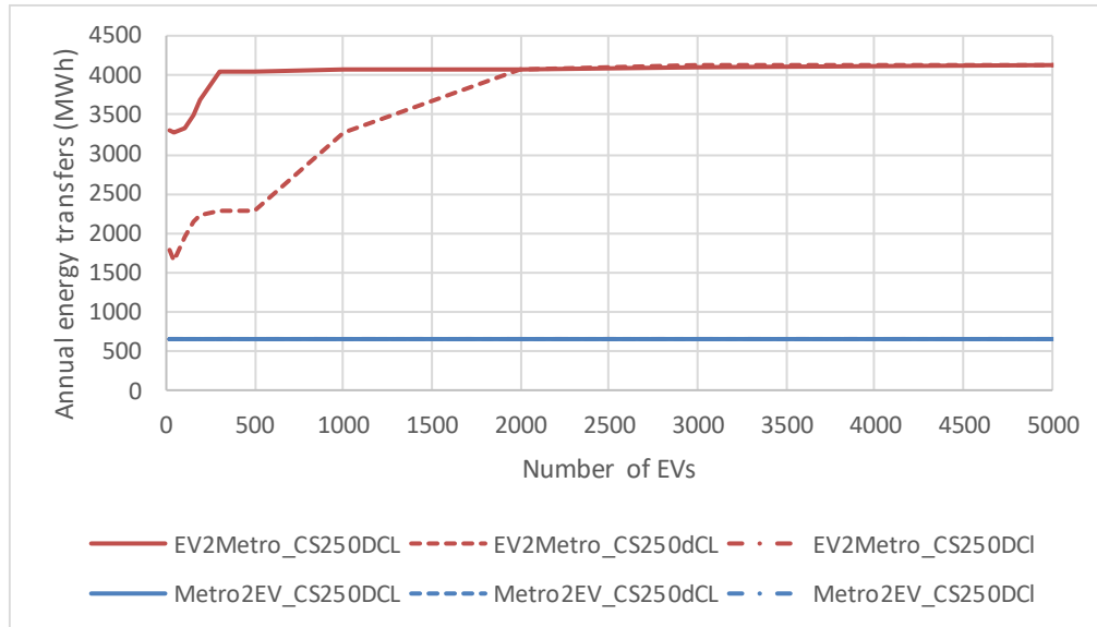
FIG. 39. ANNUAL ENERGY TRANSFERS METRO-EV FOR CS 250DCL , CS 250DCL AND CS 250DCL , AND DIFFERENT LEVELS OF EV PENETRATION.
