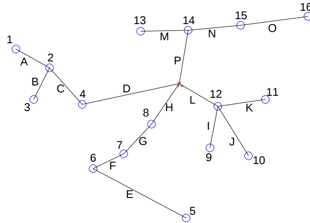
FIG. 9. DISTRICT ELECTRIC NETWORK: CASE STUDY C.
