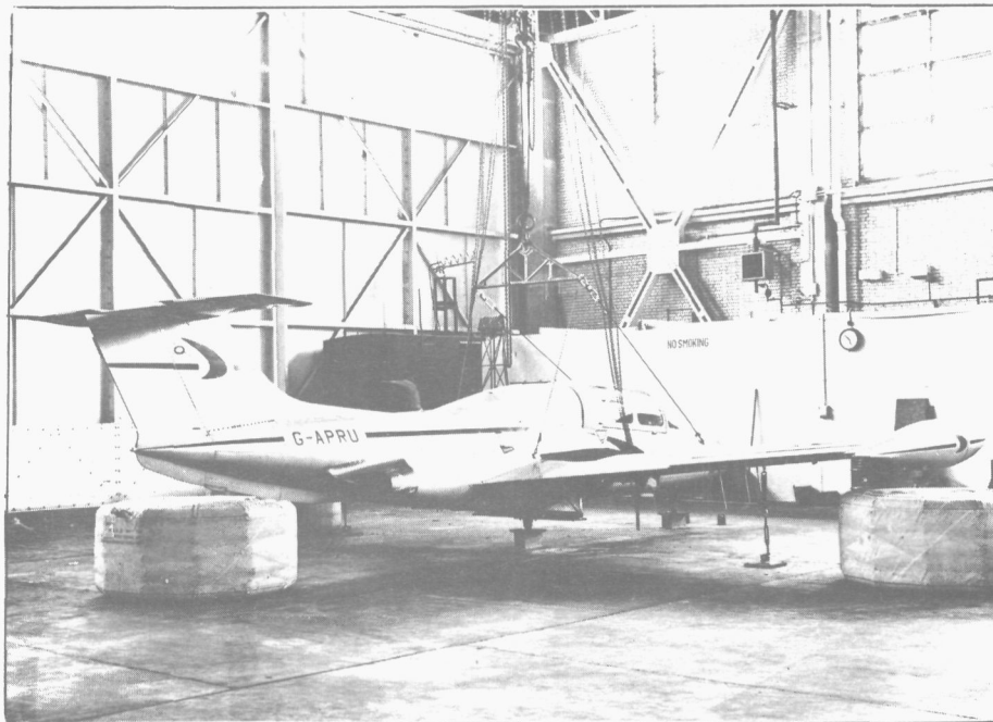
FIG. 7. VIEW OF THE AIRCRAFT ON THE ROLLING YAWING RIG
