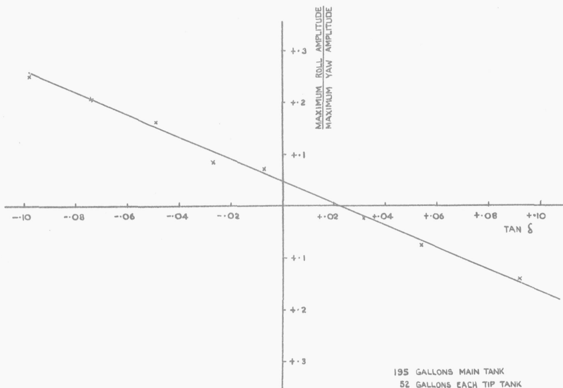
FIG. 12. GRAPH OF RATIO OF MAXIMUM ROLL AMPLITUDE TO MAXIMUM YAW AMPLITUDE PLOTTED AGAINST \tan \delta FOR FUEL CONDITION 3.
