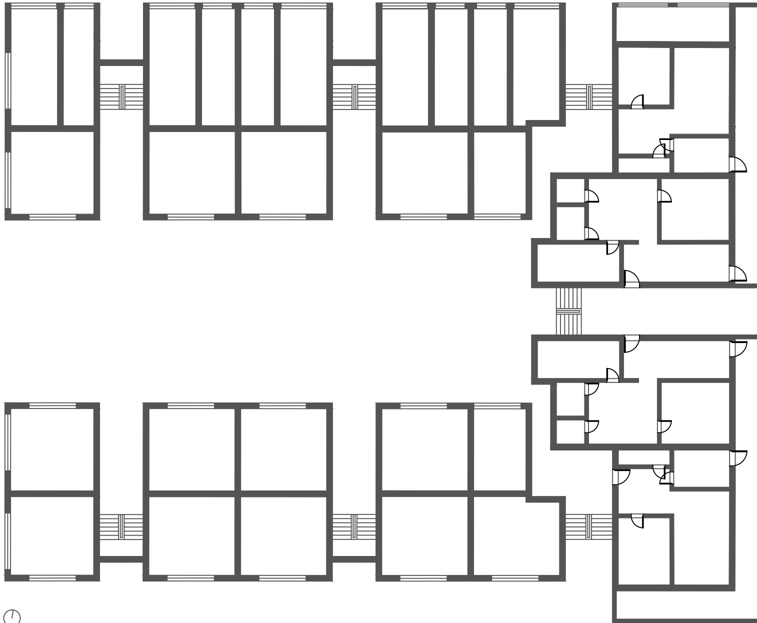
ground floor
