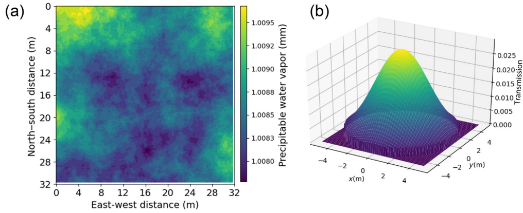
Fig. 3 (a) Colormap of the output of ARIS for a 32 m × 32 m sky window converted to PWV with Eq. (1). (b) The truncated Gaussian that is used as the telescope beam shape in the model. The volume of the Gaussian is normalized to unity, and it is truncated at a radius of 5 m, where its height is 10% of its peak height (Video 1, Mp4, 1070 KB [URL: https://doi.org/10.1117/1.JATIS.8.2.028005.1 ]).
